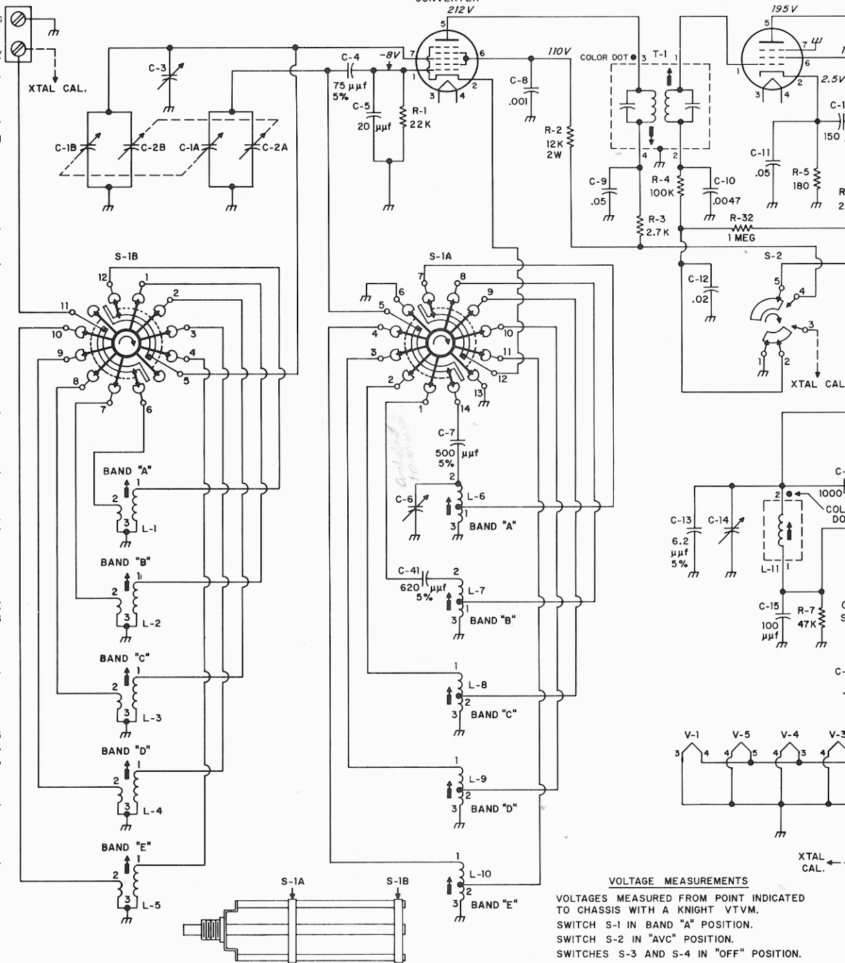
BAND SELECTOR SWITCH S-1
