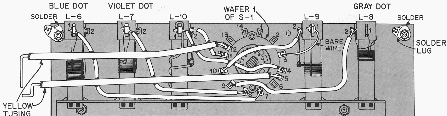
FRONT OF S-1 REMOVED FOR CLARITY
